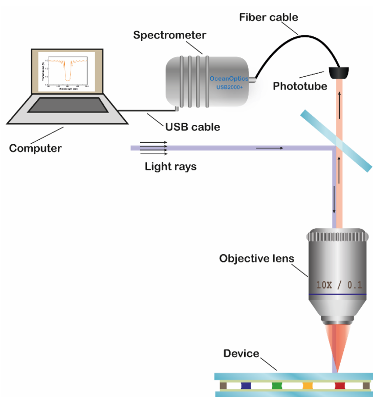
Figure S1: Schematic illustration of the experimental arrangement used to record reflection spectra. Reflection spectra were captured using an Ocean Optics USB 2000+ spectrometer connected to the phototube of an optical microscope with a reflection arm.
